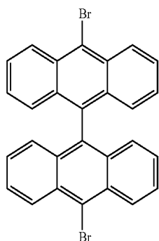
10:10'dibromo-[9,9']bianthracenyl
