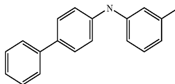
Biphenyl-4-yl-m-tolyl-amine
