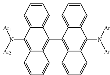
10,10'diamino-[9,9']dianthracenyl materials
